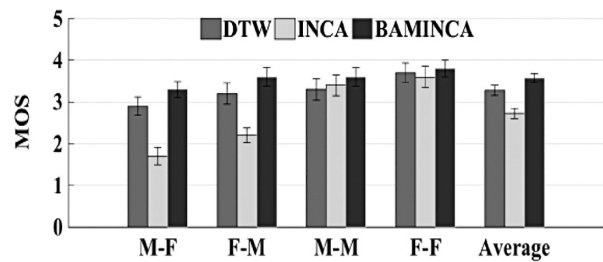
(a) MOS Test
