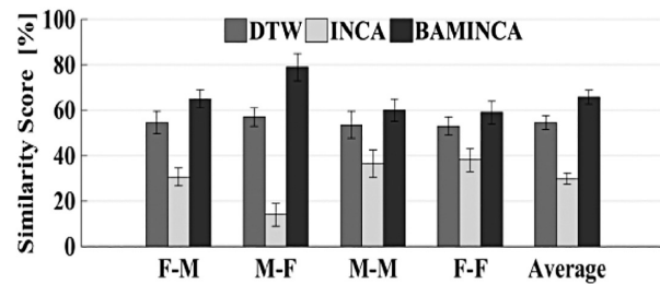
(b) Similarity Preference Test
